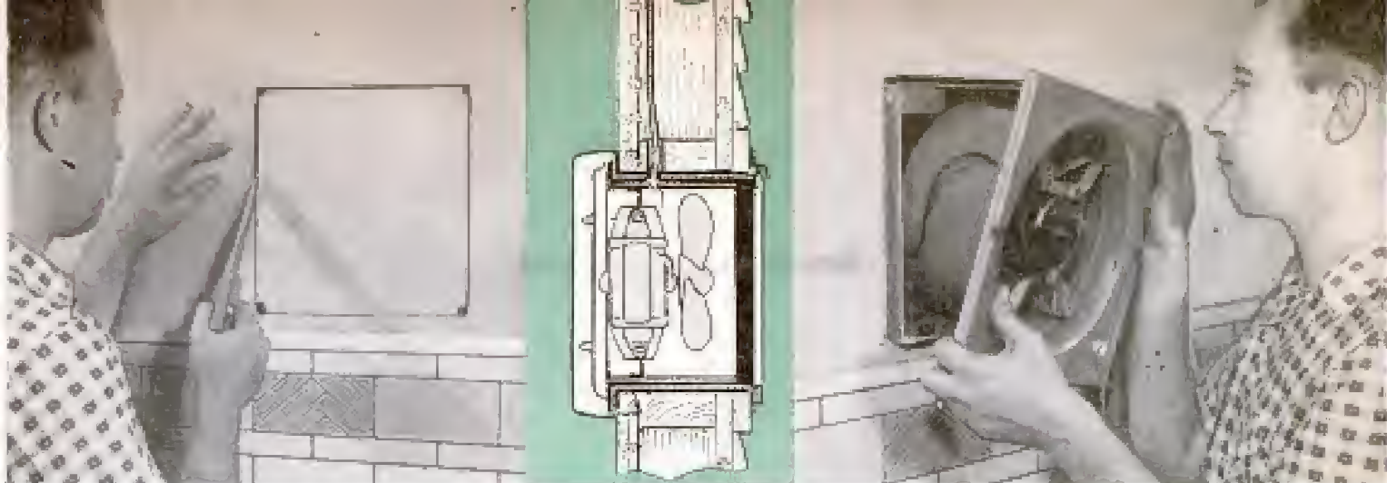
Photos show steps in mounting typical fan in outside wall. Square sheet-metal outer housing, containing lift-up door and built-in switch, bolts to fan assembly in pillbox fashion. Features plastic grille
